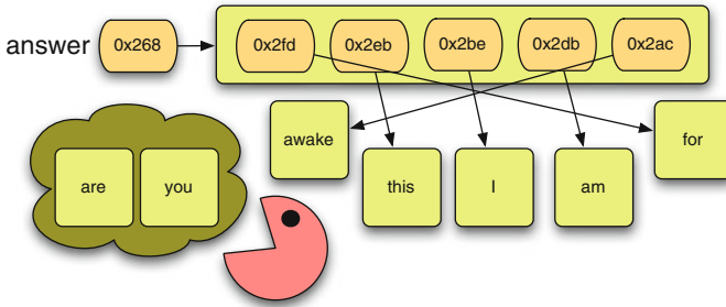
Fig. 3.5 A mutated list object
