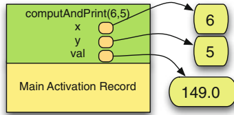
Fig. 5.3 The run-time stack for Example 5.2
