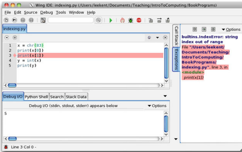
Fig. 1.22 An index out of range error
