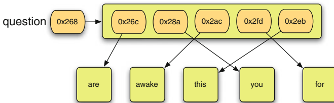
Fig. 3.4 A list object
