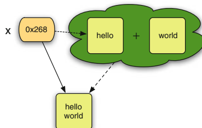
Fig. 4.6 Concatenation of two strings
