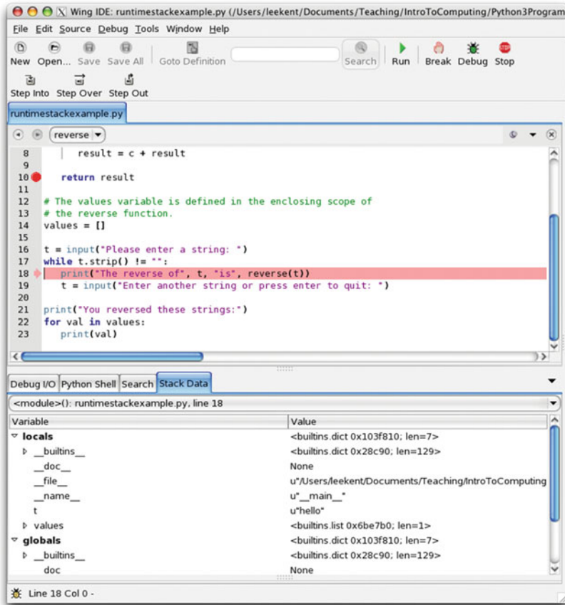
Fig. 5.2 The run-time stack in the wing IDE
