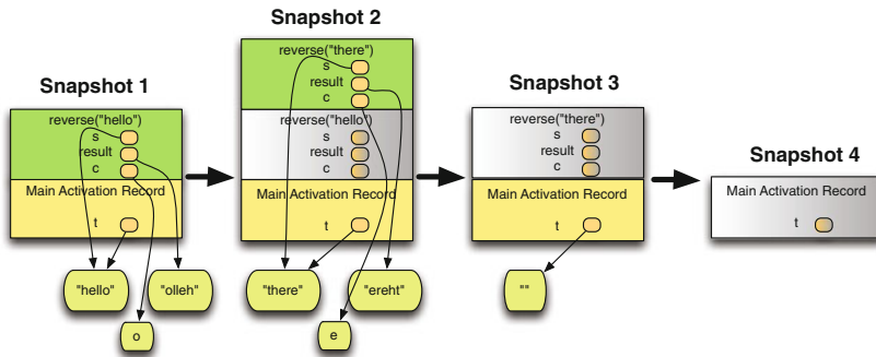
Fig. 5.1 The run-time stack
