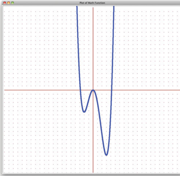
Fig. 4.5 The plot of g(x) = x^4/4 - x^3/3 - 3x^2
